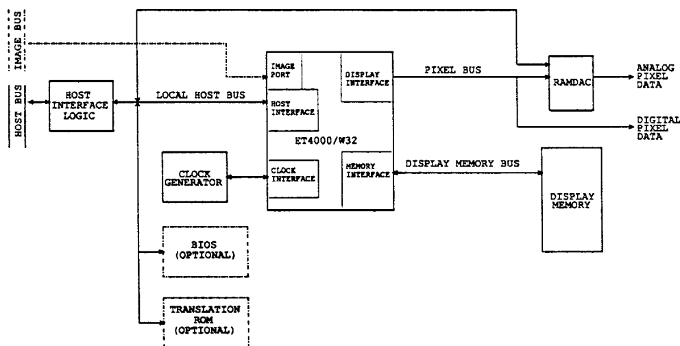
Figure 6.1-1 Board Level Block Diagram
